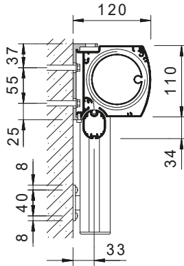
Wandmontage
